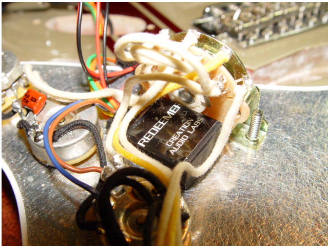
4 – Redeemer Detail
