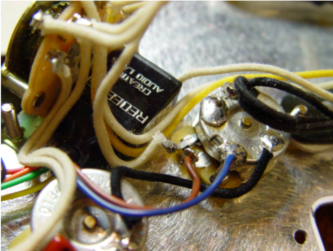
5 - Volume Pot Connection
