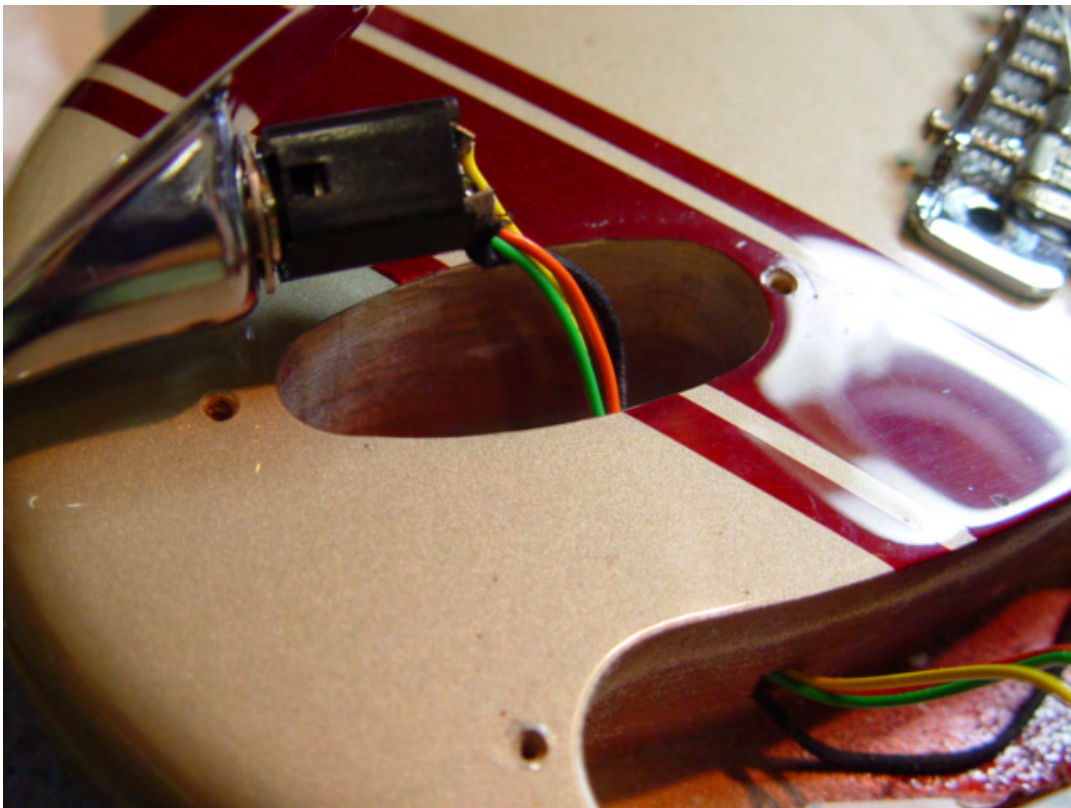
2 - Strat Jack Side View
